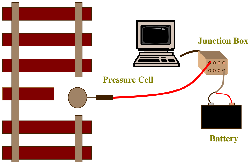
FIGURE 3a. Pressure Cell Measurement Configuration.
