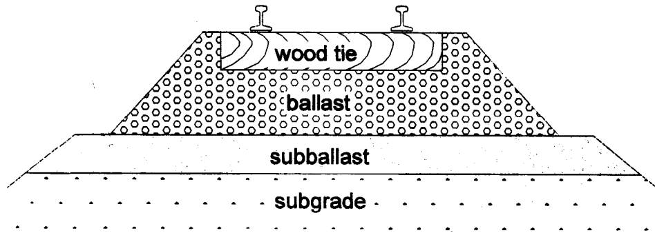
FIGURE 1a. Typical All-Granular Ballast Trackbed.
