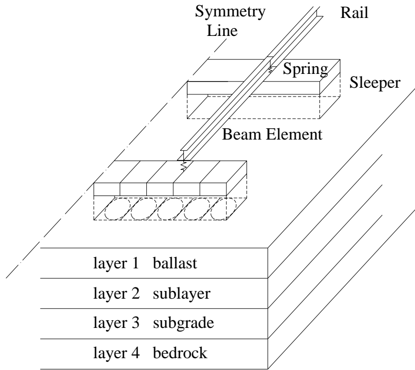
FIGURE 10. Railroad Track Model.
