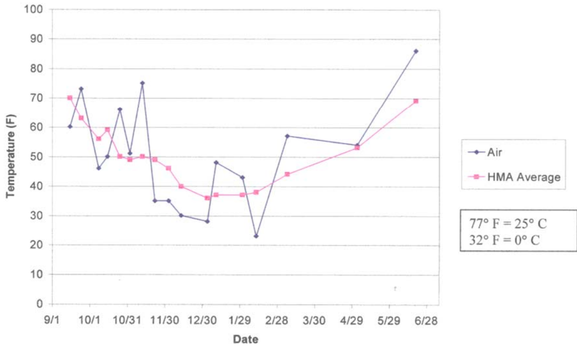
FIGURE 9. HMA Temperature Versus Air Temperature.
