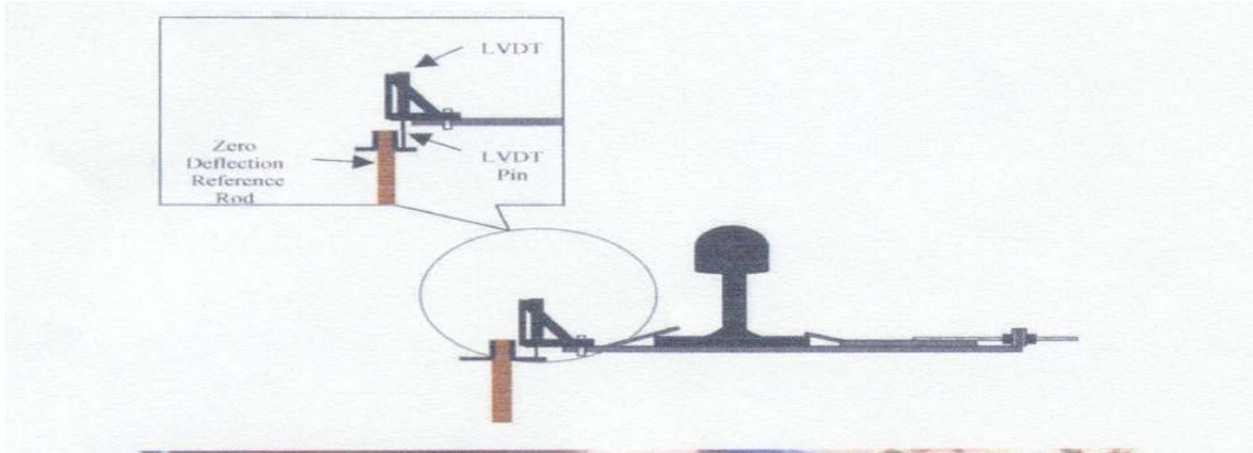
FIGURE 4a. LVDT Measurement Configuration.
