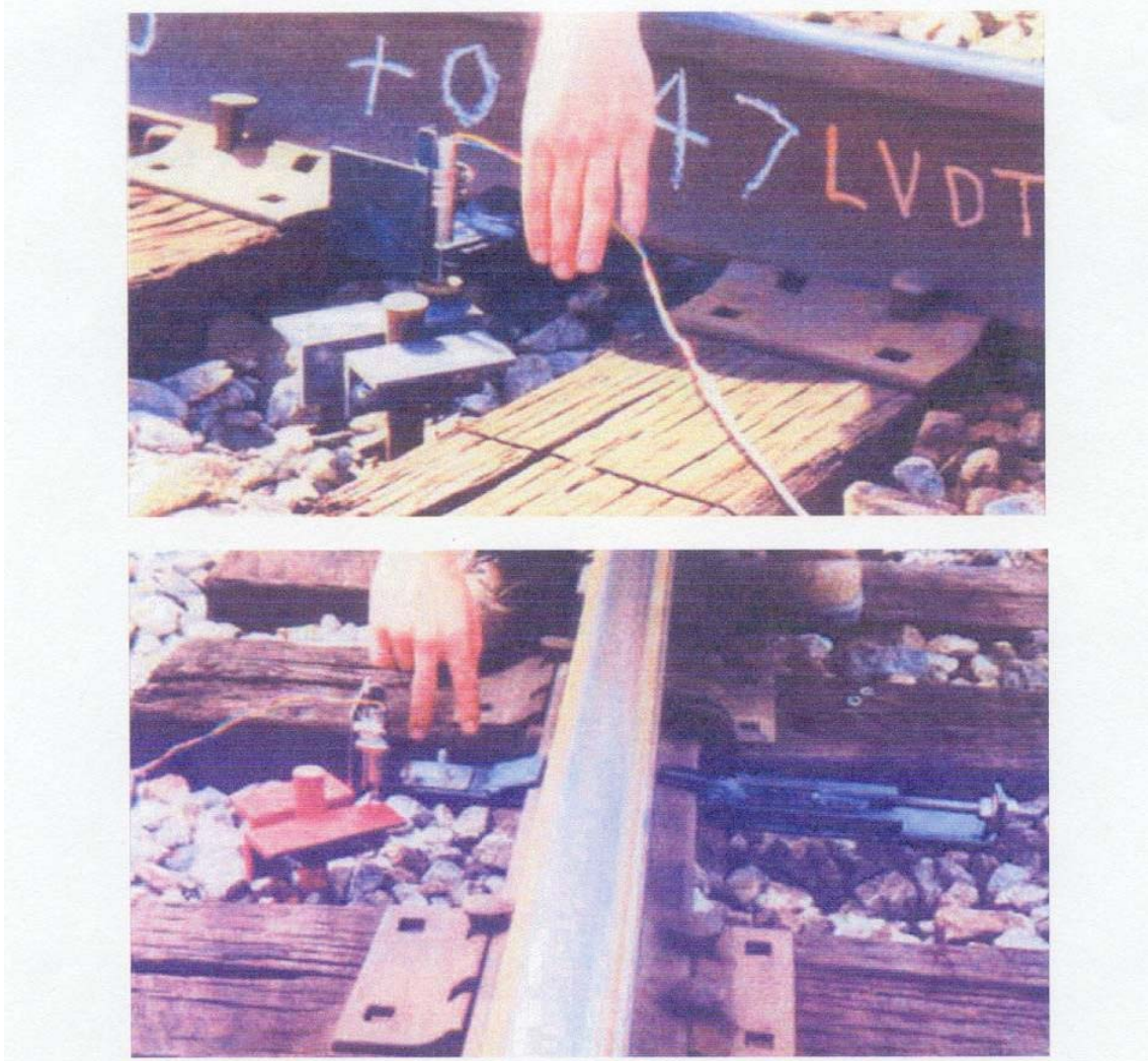
FIGURE 4b. In-track View of LVDT Deflection Testing.
