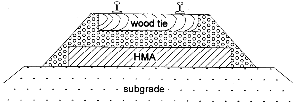
FIGURE 1b. Typical Hot Mixed Asphalt (Underlayment) Trackbed.
