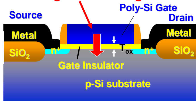
MOS Transistor-Logic Switches
