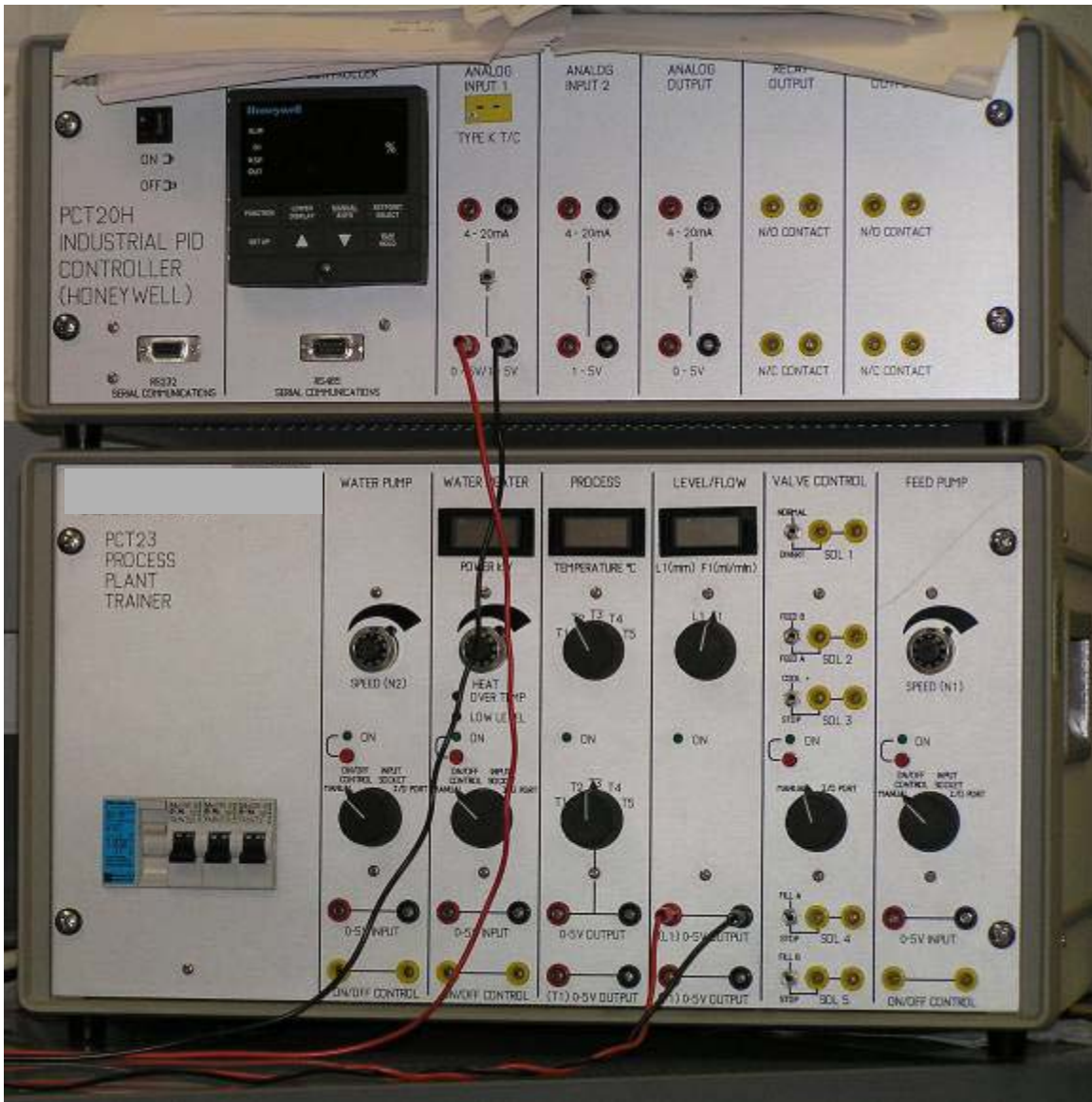
Figure 4. Control panel and interface board for the plant trainer.
