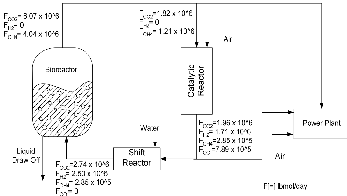
Figure 2: Flowrates (in lbmol/day) of Major Components using Initial S1 Guesses
