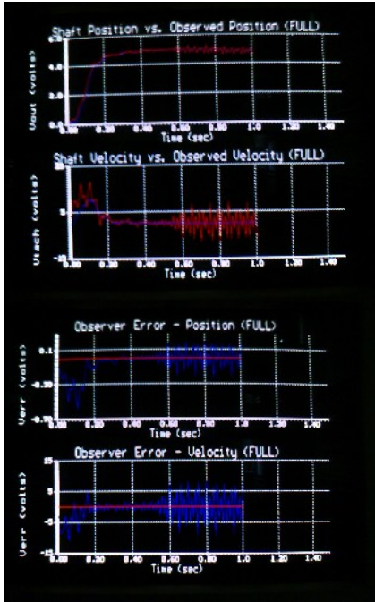
Full Observer - Conservative Gains K_{O0} = 0.83 , K_{O1} = 4.999
