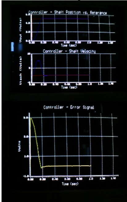
Full Order Observer w/ Deadbeat Gains K_{O0} = 1.95 , K_{O1} = 29.8
