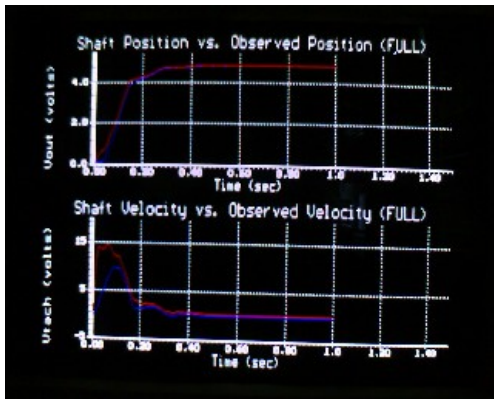
Full Observer - Conservative Gains K_{O0} = 0.83 , K_{O1} = 4.999
