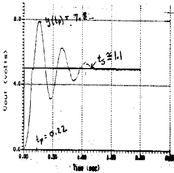
Shaft Position vs. Reference
