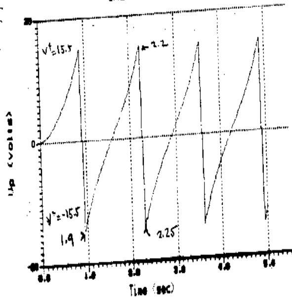
Shaft Position
